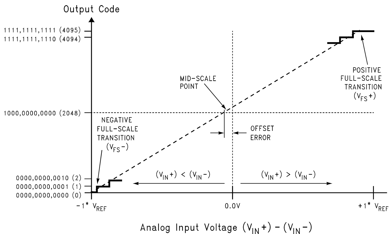
Figure 2. Transfer Characteristic
